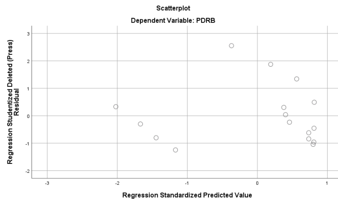
Gambar 1. Scatterplots
